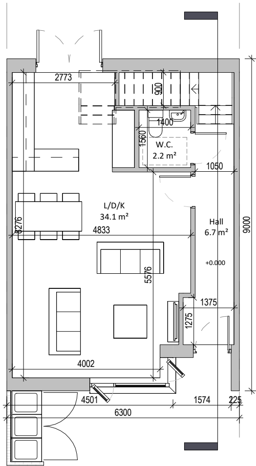
1 Ground Floor Plan 1 : 100
