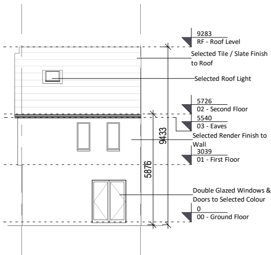
5 Rear Elevation 1 : 200
