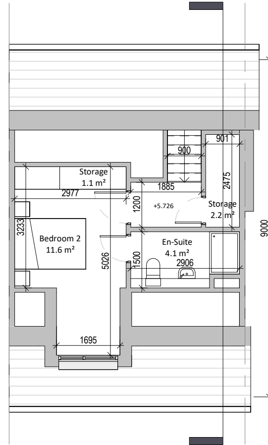
3 Second Floor Plan 1 : 100
