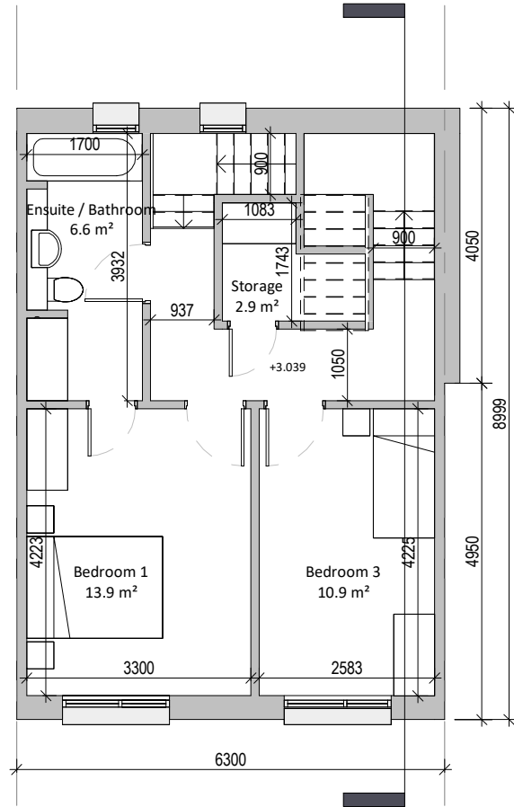
2 First Floor Plan 1 : 100
